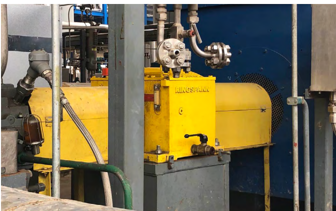
Housing Freewheel FH 2000 in hydraulic turbine pump
